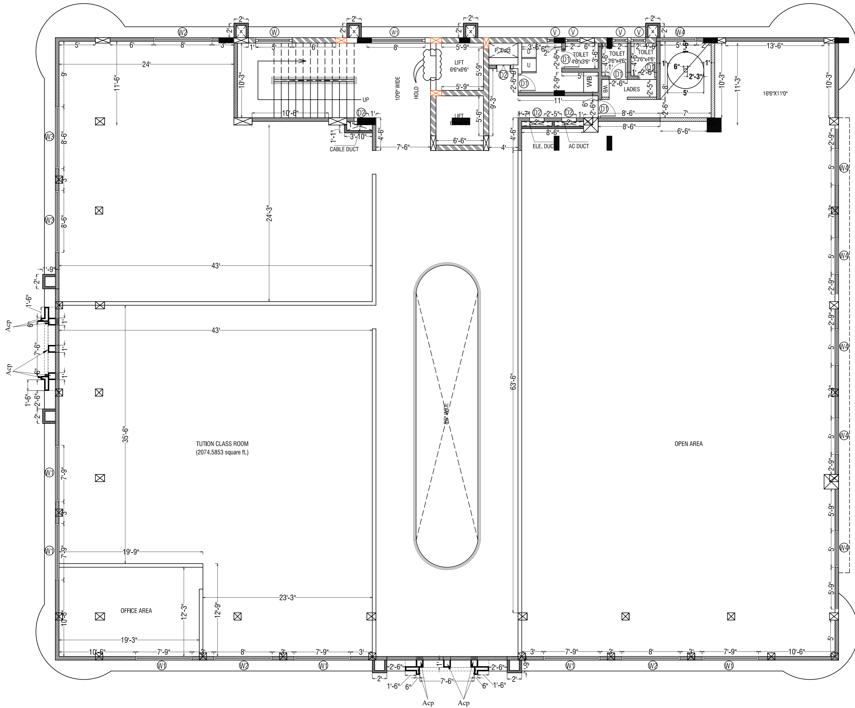
TEERRACE FLOOR PLAN
